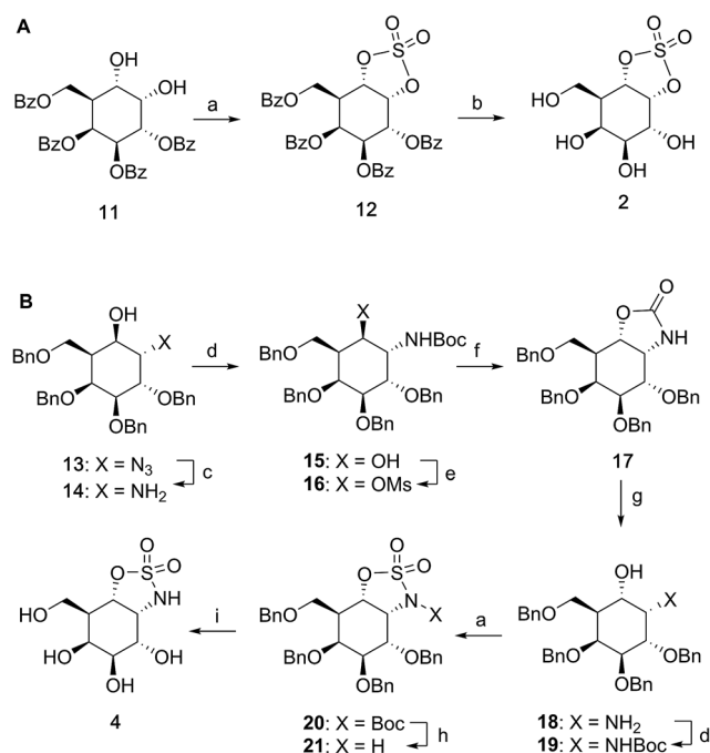
Scheme 1 Synthesis of \alpha -D-galactose configured cyclosulfate 2 (A) and cyclosulfamidate 4 (B). Reagents and conditions: (a) (i) \text{SOCl}_2 , \text{Et}_3\text{N} , imidazole, DCM, 0^\circ\text{C} ; (ii) \text{RuCl}_3 , \text{NaIO}_4 , \text{CCl}_4 , MeCN, 0^\circ\text{C} , 3 h, 12 : 56% and 20 : 59%; (b) \text{NH}_3 , MeOH, rt, 3 h, 34%; (c) \text{PtO}_2 , \text{H}_2 , THF, rt, 4 h, 99%; (d) \text{Boc}_2\text{O} , \text{Et}_3\text{N} , DCM, rt, 16 h, 15 : 93% and 19 : 99%; (e) imidazole, MsCl, \text{Et}_3\text{N} , \text{CHCl}_3 , rt, 16 h; (f) DMF, 120^\circ\text{C} , 2 days, 47% over 2 steps; (g) 1 M NaOH, EtOH, 70^\circ\text{C} , 3 h, to rt, 16 h, 86%; (h) TFA, DCM, rt, 16 h, 71%; (i) \text{Pd}(\text{OH})_2 , \text{H}_2 , MeOH, rt, 18 h, 57%.
