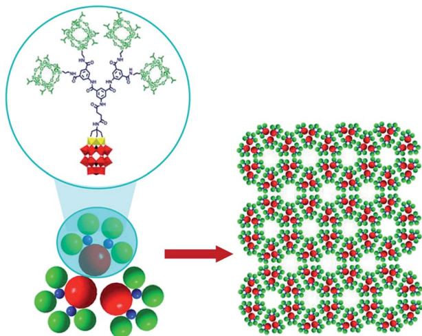
Fig. 9 The honeycomb monolayer grid formed by (\text{TBA})_6[\text{P}_2\text{W}_{15}\text{V}_5\text{-O}_{62}(\text{POSS})_4] . TBA ions are omitted for clarity. Colour code: W, red; V, yellow; P, black polyhedra. Adapted with permission from ref. 55a. Copyright 2018 American Chemical Society.
