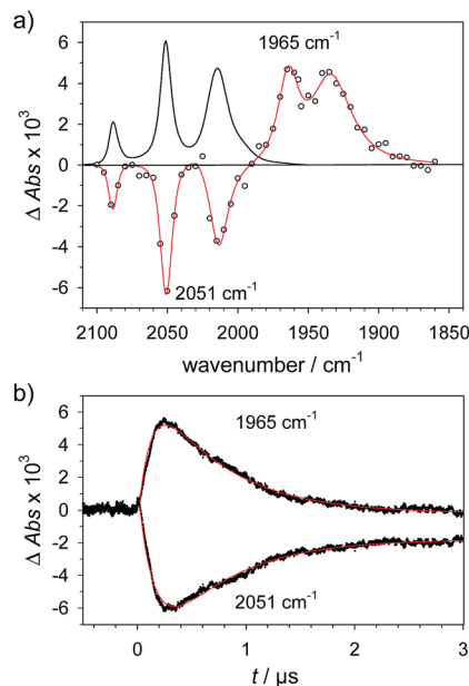
Fig. 5 (a) Transient IR spectrum 0.3 \mu\text{s} after excitation (O, \color{red}{\text{---}} ) and normalized IR spectrum of the starting state ( \text{---} ) for formation of \mathbf{1H} by reduction of \mathbf{1H}^+ (obtained by protonation of \mathbf{1} with 2.6 mM \text{Cl}_2\text{BSA} ) with flash-quench generated [\text{Ru}(\text{dmb})_3]^+ in acetonitrile. (b) Kinetic traces ( \cdots ) and fits ( \color{red}{\text{---}} ) monitoring pseudo-first order formation of \mathbf{1H} ( 1965\text{ cm}^{-1} ) and bleach of \mathbf{1H}^+ ( 2051\text{ cm}^{-1} ) followed by pseudo-first order decay of \mathbf{1H} by protonation with \text{Cl}_2\text{BSA} and charge recombination with \text{TTF}^+ .
