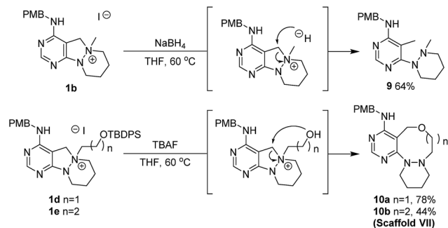
Scheme 5 Exploration of C–N bond cleavage pathway (iv) for scaffold VII.
