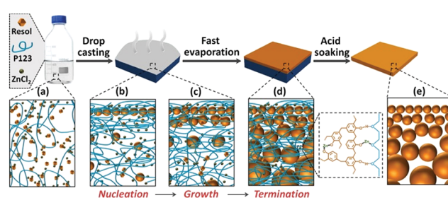
Fig. 4 Illustration of the formation of the gradient nanoporous phenolics. (a) Casting the ethanolic solution of resol, P123 and \text{ZnCl}_2 onto the substrate; (b and c) heating initiated the thermopolymerization of resol and gelation of P123 with the fast evaporation of ethanol, leading to the nucleation (b) and growth (c) of phenolic nanoparticles; (d) the phenolic particles were frozen in the gelled P123 with the complete evaporation of ethanol and the growth was terminated; (e) the gradient nanoporous structure was produced by removing P123 and \text{ZnCl}_2 with \text{H}_2\text{SO}_4 .
