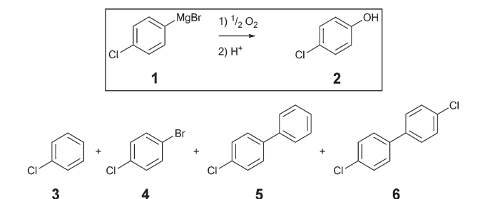
Scheme 1 Aerobic oxidation of 4-chlorophenylmagnesium bromide 1 including the desired product 2 , quenched starting material 3 and the side products 4 , 5 and 6 .
