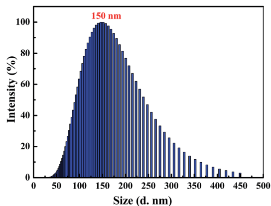
Fig. 2 Size distribution curve of luminogen 1 ( 2.0 \times 10^{-5} \text{ mol L}^{-1} ) in acetonitrile–water mixtures with f_w = 90\% .
