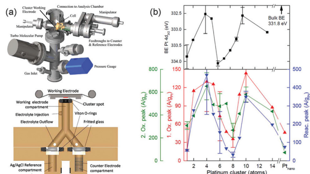
Fig. 19 (a) (top) Antechamber with cell. (bottom) Horizontal section of the cell. (b) (top) Pt 4d binding energies. (bottom) Mass activities for each EOR peak as a function of cluster size. Adapted with permission from ref. 212. Copyright 2016, American Chemical Society.
