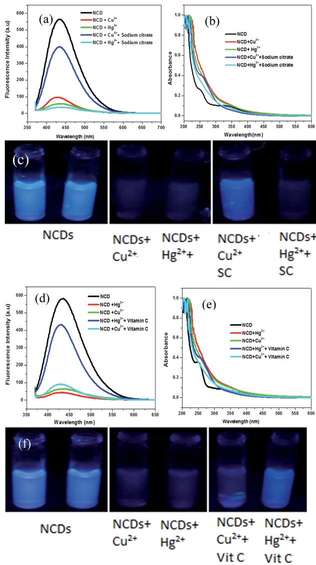
Fig. 5 (a) Fluorescence emission spectra of NCDs (2 mL) before and after addition of Hg^{2+} , Cu^{2+} ( [M^{n+}] = 50 \mu M, 10 \mu L ) and then trisodium citrate (SC = 50 \mu M, 10 \mu L ); (b) UV-visible spectrum of NCDs before and after addition of Hg^{2+} , Cu^{2+} , trisodium citrate ( [M^{n+}] and/or SC = 50 \mu M, 10 \mu L ); (c) corresponding digital photograph under 365 nm UV light; (d) fluorescence emission spectra of NCDs (2 mL) before and after addition of Hg^{2+} , Cu^{2+} , vitamin C ( [M^{n+}] and/or Vit C = 50 \mu M, 10 \mu L ); (e) UV-visible spectrum of NCDs before and after addition of Hg^{2+} , Cu^{2+} , vitamin C ( [M^{n+}] and/or Vit C = 50 \mu M, 10 \mu L ); (f) corresponding digital photograph under 365 nm UV light.
