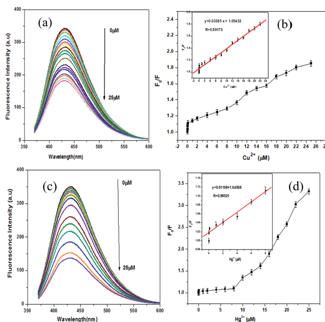
Fig. 6 (a) Fluorescence emission responses of aqueous NCDs on addition of Cu^{2+} (0–25 \mu M ) ions with excitation wavelength fixed at 360 nm; (b) plot of F_0/F vs. Cu^{2+} concentration (0–25 \mu M ), error bars are derived from three independent sets of experiments. (c) Fluorescence emission responses of aqueous NCDs on addition of Hg^{2+} (0–25 \mu M ) ions with excitation wavelength fixed at 360 nm; (d) plot of F_0/F vs. Hg^{2+} concentration (0–25 \mu M ), error bars are derived from three independent sets of experiments.
