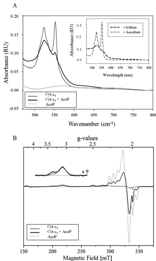
Fig. 2 (A) UV-vis spectra of 15 \mu\text{M} AcoP “as prep” (light grey), 15 \mu\text{M} reduced Cyt c_4 (dark grey), and AcoP/Cyt c_4 1 : 1 mix (15 \mu\text{M} of each in the final mixture) (black) in 20 mM NaAC buffer, pH 4.8. Inset: typical spectra of oxidized Cyt c_4 obtained after the addition of \text{K}_2\text{IrCl}_6 (black dashed line) or of reduced Cyt c_4 obtained after the addition of ascorbate (grey dashed line); (B) EPR spectra of 100 \mu\text{M} AcoP “as prep” (light grey), 100 \mu\text{M} Cyt c_4 untreated (dark grey) and AcoP/Cyt c_4 1 : 1 mix (100 \mu\text{M} of each in the final mixture) (black) in 20 mM NaAc buffer, pH 4.8. Acquisition parameters: temperature = 15 K, microwave frequency = 9479 MHz, microwave power = 0.2 mW, and modulation amplitude = 2 mT. Inset: magnification of the g_z -peak region of low-spin hemes (microwave power = 4 mW).
