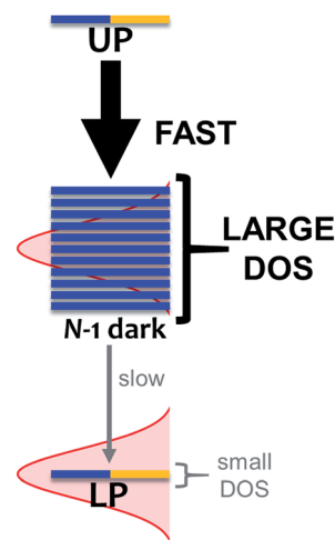
Fig. 4 Effect of DOS on vibrational-relaxation dynamics in the regime of strong coupling between N excitons and a single photon mode. For large N , decay from UP to dark states (DOS \approx (N - 1)/ exciton linewidth) is much faster compared to that from dark states to LP (DOS \approx 1/ LP linewidth) because transition rate scales with final DOS. When many modes are considered, the polariton bands have DOS that is larger but still much smaller than their dark state counterpart.
