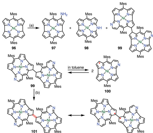
Fig. 32 Series of pyridinene derivatives. (a) 12.5 equiv. 4-Amino-4H-1,2,4-triazole, 20 equiv. NaOH, THF, reflux, 2 h, 8.6% for 97 , 28.8% for 98 , 3.3% for 99 , 32.2% for 100 ; (b) degassed DMF, N 2 , 80 °C, 30 min, 98%.
