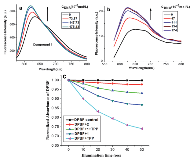
Fig. 2 Fluorescence spectra of compound 1 (a) and 2 (b) with the titration to ct-DNA. Each spectrum was recorded in pH = 7.4, 0.05 \text{ mol L}^{-1} Tris-HCl, 0.1 \text{ mol L}^{-1} NaCl buffer solution. (c) Singlet oxygen generation of 1 and 2 ( 50 \mu\text{M} ). The change of absorption of DPBF at 418 nm ( A/A_0 ) upon the irradiation time. The spectrum was recorded in DMSO.
