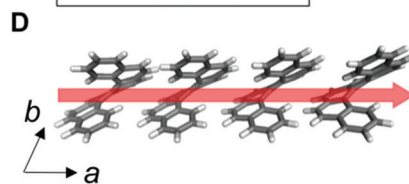
Fig. 8 Angular-dependent electron-mobility for structure 11 in the (a) ab -, (b) bc - and (c) ac -planes; (d) the adjacent translational homochiral chain (substructure type I ) with electron-mobility of 2.9 \text{ cm}^2 \text{V}^{-1} \text{s}^{-1} . The red arrow shows the highest electron-mobility direction for structure 11 .
