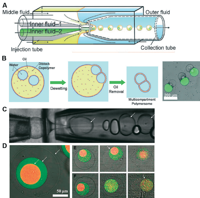
Fig. 9 Microfluidic generation of compartmentalised polymer structures. (A) Microfluidic generation of multicompartiment polymersomes using glass capillary devices. (B) Formation mechanism of multicompartiment polymersomes from double emulsion drops with multiple inner droplets and relevant fluorescence/brightfield composite image of the systems. (C) Microfluidic generation of polymersome-in-polymersome systems using glass capillary devices. (D) Confocal microscope images showing triple polymersomes. (E) Series of images showing sequential dissociation of membranes from the outermost to the middle of triple polymersome. (F) Series of images showing sequential dissociation of membranes from the innermost to the outermost of triple polymersomes. Subfigures (A) and (B) are reproduced from ref. 110 with permission from Angew. Chem. Subfigures (C) and (D) reprinted with permission from ref. 111, copyright 2011 American Chemical Society.
