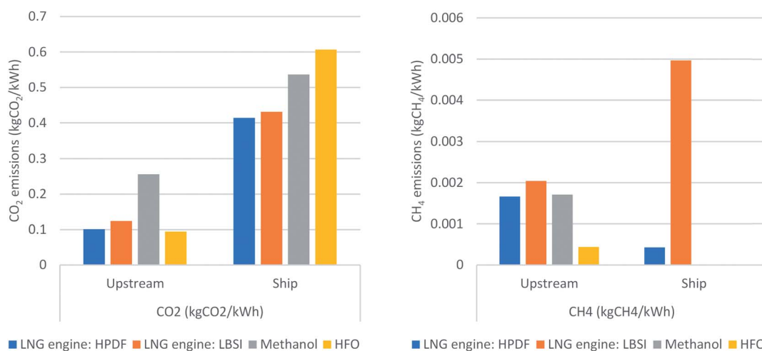
Fig. 10 CO 2 and methane emissions associated with the supply and use of 4 different fuels and engines for ships. Emissions are divided into upstream supply chain and ship usage. Source: ref. 51–61.
