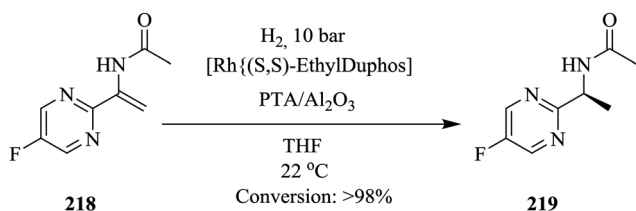
Scheme 43 Asymmetric hydrogenation in flow.
