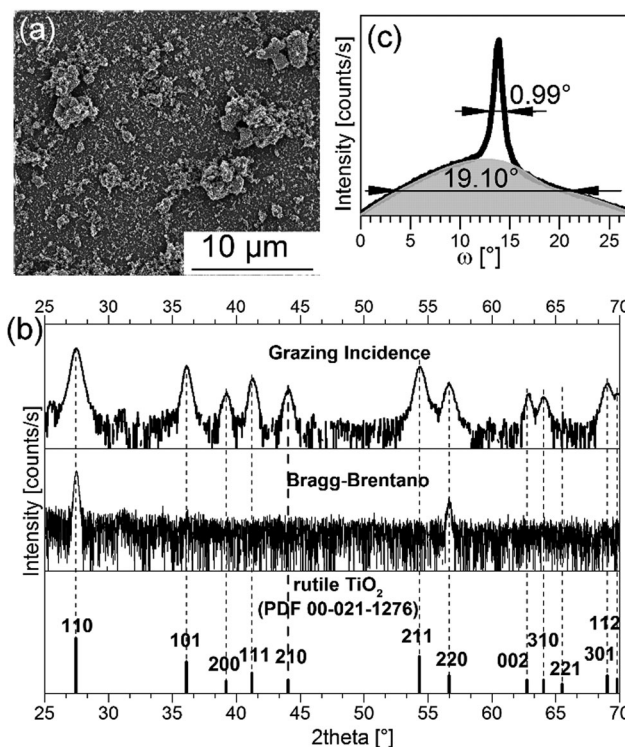
Fig. 2 (a) SEM image showing the surface of a 2 wt% S:TiO 2 nanoparticle substrate after spin coating (without FTO film). (b) Corresponding Bragg–Brentano and grazing incidence XRD patterns plotted in log scale. (c) Corresponding (110) rocking curve plotted in linear scale.
