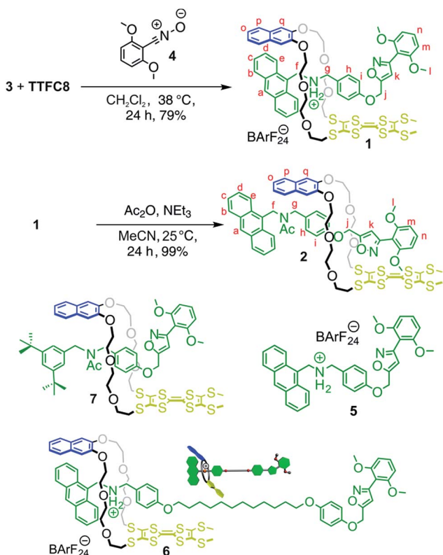
Scheme 1 Preparation of charged and non-charged [2]rotaxanes 1 and 2 ; structures of free stoppered axle 5 , [2]rotaxanes 6 and 7 .
