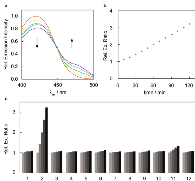
Fig. 2 FA response and selectivity of RFAP-1. Data were acquired at 37\text{ }^\circ\text{C} in 20\text{ mM} PBS ( \text{pH } 7.4 ). Excitation spectra were collected between 400 and 500\text{ nm} with emission monitored at \lambda_{\text{em}} = 510\text{ nm} . (a) Excitation ratiometric response of 10\text{ }\mu\text{M} RFAP-1 to 100\text{ }\mu\text{M} FA. Excitation spectra are shown at 0 , 30 , 60 , 90 , and 120\text{ min} (red, yellow, green, blue, and purple traces, respectively) after addition of FA. (b) Quantification of 470/420\text{ nm} excitation ratio over time. (c) Excitation ratiometric response of 10\text{ }\mu\text{M} RFAP-1 to biologically relevant RCS and related molecules. Bars represent relative 470/420\text{ nm} excitation ratios at 0 , 30 , 60 , 90 , and 120\text{ min} after the addition of a given analyte. The data shown are for a concentration of 100\text{ }\mu\text{M} for all species unless otherwise denoted. Legend: (1) PBS; (2) FA; (3) acetaldehyde; (4) pyruvate; (5) glucose, 1\text{ mM} ; (6) 4-HNE; (7) dehydroascorbate; (8) oxaloacetate; (9) glucosone; (10) acrolein; (11) methylglyoxal; (12) methylglyoxal, 10\text{ }\mu\text{M} .
