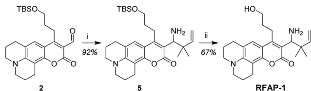
Scheme 4 Synthesis of RFAP-1. Reagents and conditions: (i) \text{NH}_3 , \text{MeOH} , 0\text{ }^\circ\text{C} , then prenylboronic acid, rt, 10 h; (ii) \text{AcOH} , \text{H}_2\text{O} , rt, 14 h.
