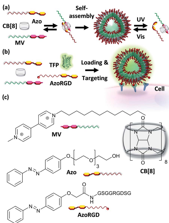
Fig. 1 (a) A supramolecular amphiphile is formed as a ternary complex between CB[8], methyl viologen with a hydrophobic alkyl chain (MV) and azobenzene with a hydrophilic oligo(ethylene glycol) chain (Azo). (b) Cell targeting is provided by including AzoRGD peptide ligands, while the vesicles can be loaded with teal, yellow and red fluorescent proteins (TFP, YFP, TagRFP) as cargo (TFP is shown). (c) Molecular structures of MV, Azo, AzoRGD and CB[8].
