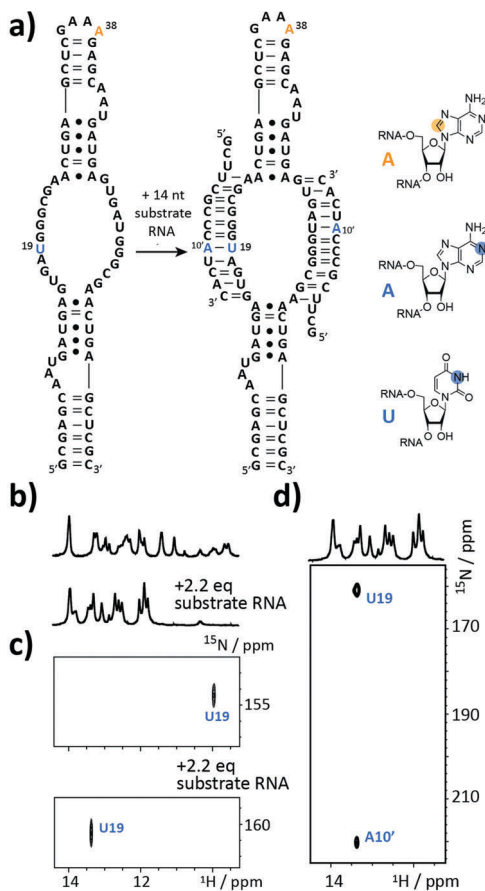
Fig. 3 Stable isotope (SI) labelling of the 72 nt box C/D guide ssR26 RNA. (a) Secondary structure representation with residues U19 and A38 carrying a 3- ^{15}\text{N} - and an 8- ^{13}\text{C} -label highlighted in blue and orange, respectively. The 14 nt substrate RNA was modified with a 1- ^{15}\text{N} -adenosine label (A10', highlighted in blue). (b) Imino proton region of ^1\text{H} NMR spectrum before and after addition of 2.2 eq. substrate RNA. (c) ^1\text{H} - ^{15}\text{N} -HSQC spectra before and after addition of 2.2 eq. substrate RNA. (d) HNN COSY experiment to confirm the intermolecular Watson Crick base pair between U19 and A10'. Orange dot = ^{13}\text{C} , blue dot = ^{15}\text{N} .
