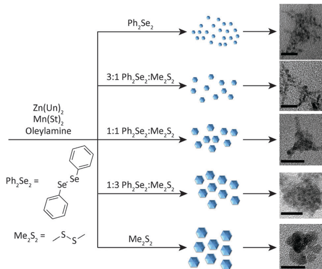
Fig. 1 General synthetic scheme for formation of \text{Mn}^{2+} -doped \text{ZnSe}_{1-x}\text{S}_x NCs. In the reaction, zinc undecylate, \text{Zn}(\text{Un})_2 , manganese stearate, \text{Mn}(\text{St})_2 , and a mixture of diphenyl diselenide and dimethyl disulphide (or diphenyl disulphide) are combined and heated to reaction temperature in an alkylamine under an inert atmosphere. Depending on the ratio of diselenide to disulphide, NCs of different shapes and sizes are obtained. Images of samples 1–5 are shown. Scale bars are 20 nm.
