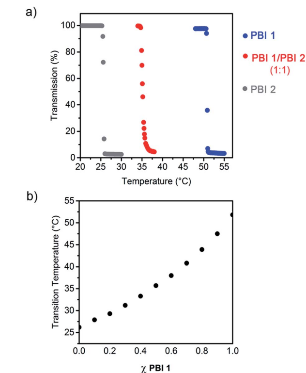
Fig. 2 (a) Transmission at 800 nm of aqueous solutions ( 2.5 \times 10^{-4} M) of PBI 1 , PBI 2 and PBI 1/PBI 2 (1 : 1) as a function of the temperature. Heating rate 0.1 \text{ }^\circ\text{C min}^{-1} . (b) Phase transition temperatures for PBI 1/PBI 2 aggregates ( 2.5 \times 10^{-4} M) as function of the molar fraction ( \chi ) of PBI 1 .
