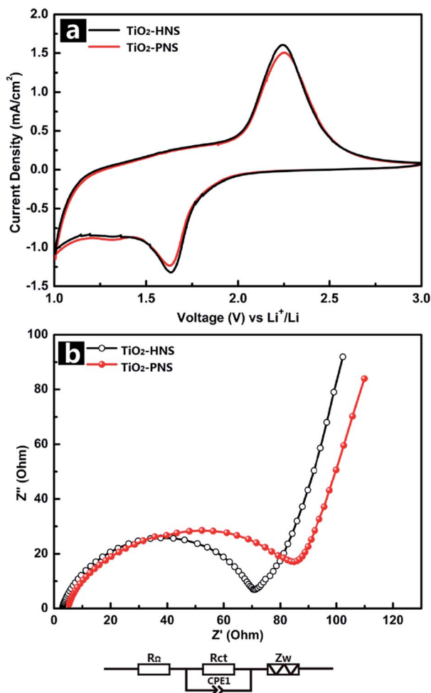
Fig. 4 (a) Cyclic voltammograms profiles of the TiO 2 -HNSs and TiO 2 -PNSs at a scan rate of 1 mV s -1 between 1.0 V and 3.0 V for the first cycle, and (b) electrochemical impedance spectra (EIS) of the TiO 2 -HNSs and TiO 2 -PNSs ( R_n : external resistance, R_{ct} : charge transfer resistance, CPE1: constant phase element, Z_w : Warburg impedance).
