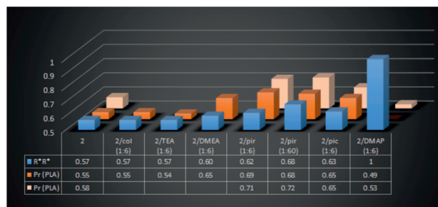
Fig. 10 The relationship between the fraction of homochiral species for 2/amine and the heteroselectivity of rac -LA polymerization with ( S,S )-2 in toluene at 40 °C (orange) and room temperature (pale orange).
