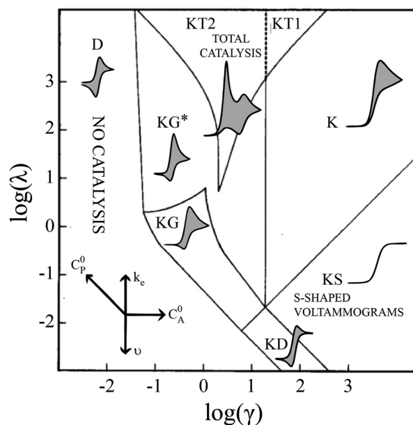
Fig. 1 Kinetic zone diagram and simulated CV waveforms for the catalytic EC' mechanism of the one electron reduction of substrate via a redox catalyst mediator. Reprinted with permission from ref. 5.
