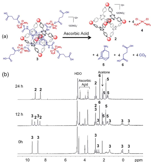
Fig. 2 (a) Chemical representation of the reduction of 3 by ascorbic acid and (b) ^1\text{H} NMR (400 MHz, R.T.) spectra showing reduction of 3 ( 0.8 \text{ mM} ) by ascorbic acid ( 8 \text{ mM} ) in deuterated PBS over 24 h at 37^\circ\text{C} .
