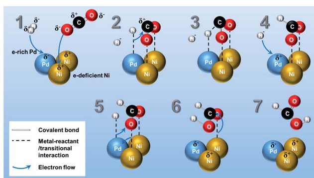
Scheme 1 A proposed reaction mechanism of selective formation of HCOOH from CO 2 hydrogenation over PdNi bimetallic surface. The \delta^+ / \delta^- signs in the illustration represent the localized electron charge in the molecules or bimetallic structure.
