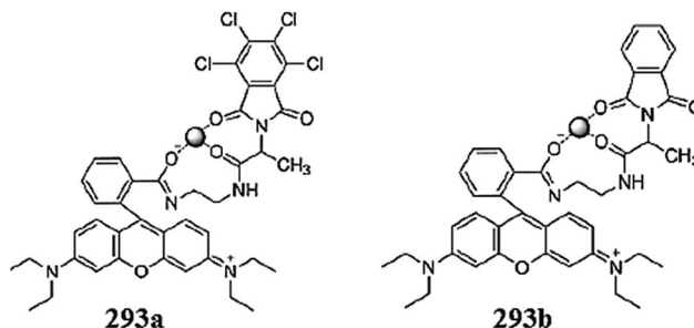
Fig. 257 Chemical structure of the ligand–Hg 2+ complexes.
