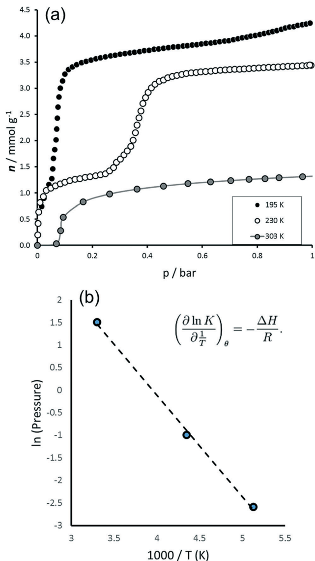
Fig. 1 Adsorption of CO 2 on MIL-53(Fe) to 1 bar. (a) Isotherms to 1 bar at 195 K, 230 K and 303 K. (b) Van't Hoff plot.
