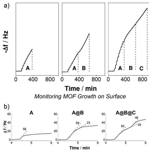
Fig. 23 A quartz crystal microbalance (QCM) can be used to monitor (a) the stepwise deposition and growth of a ternary MOF thin film, A@B@C, on a surface, and (b) the distinct sorption profiles for films of varying compositions, with stepped sorption curves suggesting mono-, bi- or tri-layer MOF thin film structures. Reprinted (adapted) with permission from ref. 78. Copyright (2013) John Wiley and Sons.
