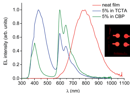
Fig. 10 Electroluminescence spectra of OLEDs incorporating \text{PtL}^2\text{Cl} as a neat film or doped in TCTA or CBP as the emitting layer at 8 V. Photo of the NIR-OLEDs (inset).
