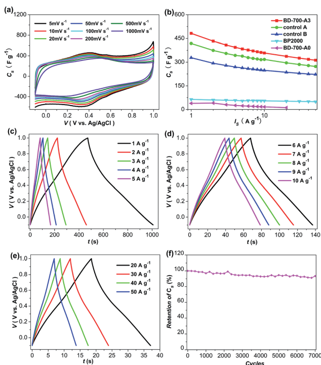
Fig. 4 Electrochemical performance of BD-700-A3 based on the three-electrode system: (a) CVs at various scan rates; (b) C_s at various current densities, compared with commercially available carbon BP2000 and some other bean dregs derived carbons; (c–e) galvanostatic charge/discharge curves collected at various current densities ( I_s ); (f) capacitance retention measured at 5 \text{ A g}^{-1} .
