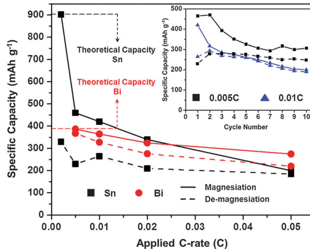
Fig. 2 Magnesianion/de-magnesiation capacities for Sn/Mg (■ black) and Bi/Mg (● red) half-cells at various C-rates. All half-cells were tested using an organohaloaluminate electrolyte. Inset – 10 cycles of a Sn/Mg half-cell at 0.005 C (■ black) and 0.01 C (▲ blue) rates in the same electrolyte.
