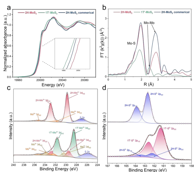
Figure 2. (a) XANES spectra & (b) k^2 -weighted Fourier transformed EXAFS spectra of the Mo K-edge of the as-prepared and standard MoS 2 samples; (c) Mo 3d XPS spectra & (d) S 2p XPS spectra of as prepared 2H- and 1T'-MoS 2 .
