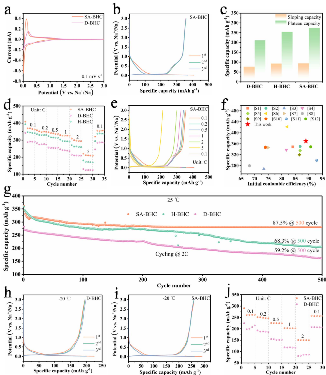
Fig. 3 (a) CV curves of D-BHC and SA-BHC at 0.1 \text{ mV s}^{-1} . (b) GCD profiles of SA-BHC at 0.1C. (c) Comparison of slope and plateau capacities among D-BHC, H-BHC, and SA-BHC. (d) Rate performance from 0.1 to 5C. (e) GCD profiles of SA-BHC at rates from 0.1 to 5C. (f) Comparison of the reversible capacity and ICE of SA-BHC with those of reported bamboo-derived HC anodes for SIBs. (g) Long-term cycling performance at 2C. (h, i) GCD profiles of D-BHC and SA-BHC at 0.1C measured at room temperature and -20^\circ\text{C} . (j) Rate capability of D-BHC and SA-BHC at -20^\circ\text{C} .
