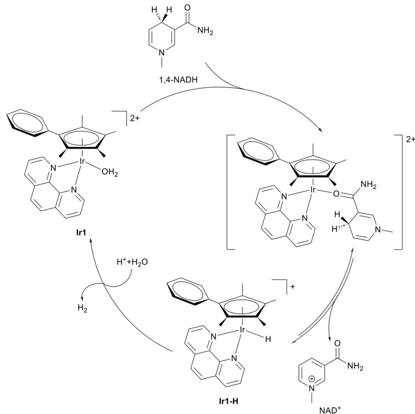
Fig. 6 Chemical structure of [(\eta^5\text{-C}_5\text{Me}_4\text{C}_6\text{H}_5)\text{Ir}(\text{phen})(\text{H}_2\text{O})]^{2+} ( Ir1 ) and its catalytic conversion of NADH to \text{NAD}^+ by hydride transfer.
