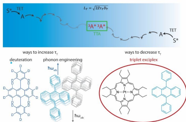
Figure 6: Top: Efficient solid-state TTA-UC requires triplets that can diffuse over long distances. The diffusion length ( L_T ) can be enhanced by either increasing the diffusion coefficient ( D_T ) or triplet lifetime ( \tau_T ). Bottom: \tau_T is a crucial parameter for efficient annihilators and it can be increased, for example, by tuning the intramolecular and intermolecular vibrational modes (deuteriation and phonon engineering, respectively) or ensuring that triplet excimers/exciplexes are not formed.
