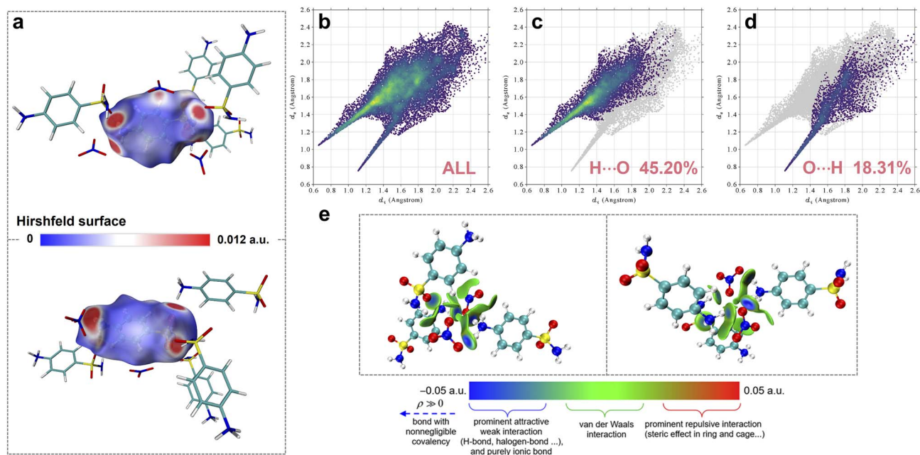
Fig. 4 The Hirshfeld isosurface of SAN in different directions (a); 2D fingerprint plots for overall interactions and individual H...O/O...H interactions in the crystal packing of SAN (b–d); IGMH isosurfaces of SAN in different directions (e).
