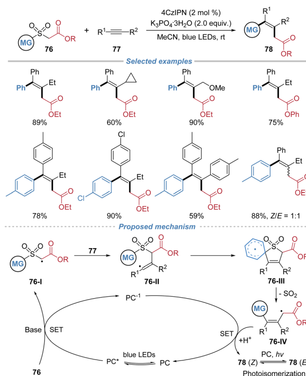
Scheme 28 Radical alkylation of alkynes using arylsulfonyl acetates as bifunctional reagents.
