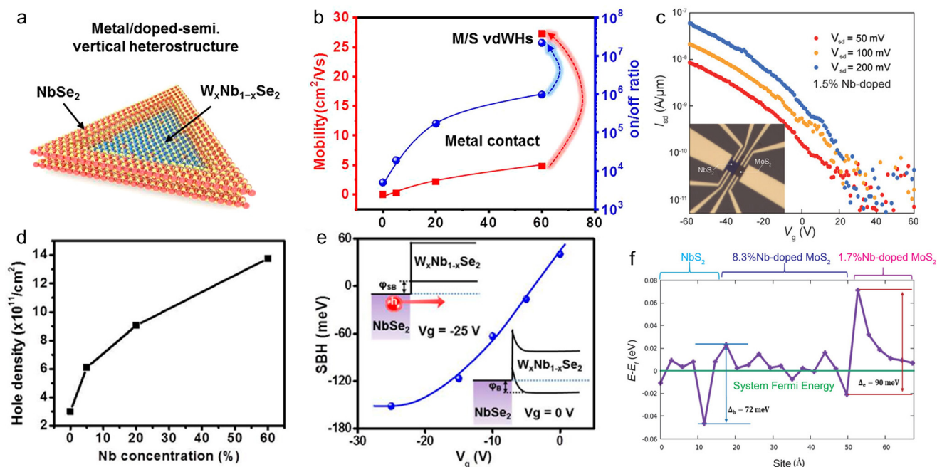
Fig. 8 Substitutional-doping-assisted ohmic contact engineering in 2D TMDs. (a) Schematic illustration of the \text{NbSe}_2 / \text{W}_x\text{Nb}_{1-x}\text{Se}_2 metal/doped-semiconductor heterostructure synthesized by one-step CVD growth. (b) Comparison of field-effect mobility (left axis) and on/off ratio (right axis) between conventional metal-contacted \text{WSe}_2 and \text{NbSe}_2 / \text{W}_x\text{Nb}_{1-x}\text{Se}_2 van der Waals heterostructures. (c) Transfer characteristics of the \text{NbS}_2 - \text{MoS}_2 lateral heterostructure, confirming stable p-type conduction. (Inset: OM image of the device). (d) Variation of hole carrier density in \text{WSe}_2 with increasing Nb incorporation (0–60%). (e) Extracted Schottky barrier height ( \Phi_{\text{SB}} ) as a function of gate voltage, showing a negative ( \Phi_{\text{SB}} ) ( \approx -0.68 \text{ eV} ) at the \text{NbSe}_2 / \text{W}_x\text{Nb}_{1-x}\text{Se}_2 interface, indicative of p-type ohmic contact formation. (f) Calculated planar-averaged electrostatic potential across the \text{NbS}_2 - \text{MoS}_2 interface, revealing a minimal potential step ( \Delta E \approx 72 – 90 \text{ meV} ) that facilitates efficient hole transport. Reproduced from ref. 43 (panels a, b, d and e) and ref. 45 (panels c and f) under Creative Commons license (CC BY).
