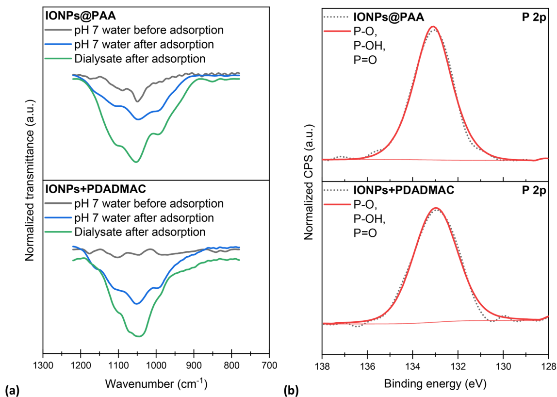
Fig. 6 (a) FTIR spectra of IONPs@PAA and IONPs+PDADMAC before and after phosphate adsorption in pH 7 water and dialysate (4 hours of contact with 300 \text{ mg P L}^{-1} phosphates). (b) P 2p peak in the XPS spectra of IONPs@PAA and IONPs+PDADMAC after phosphate adsorption in pH 7 water (4 hours of contact with 300 \text{ mg P L}^{-1} phosphates).
