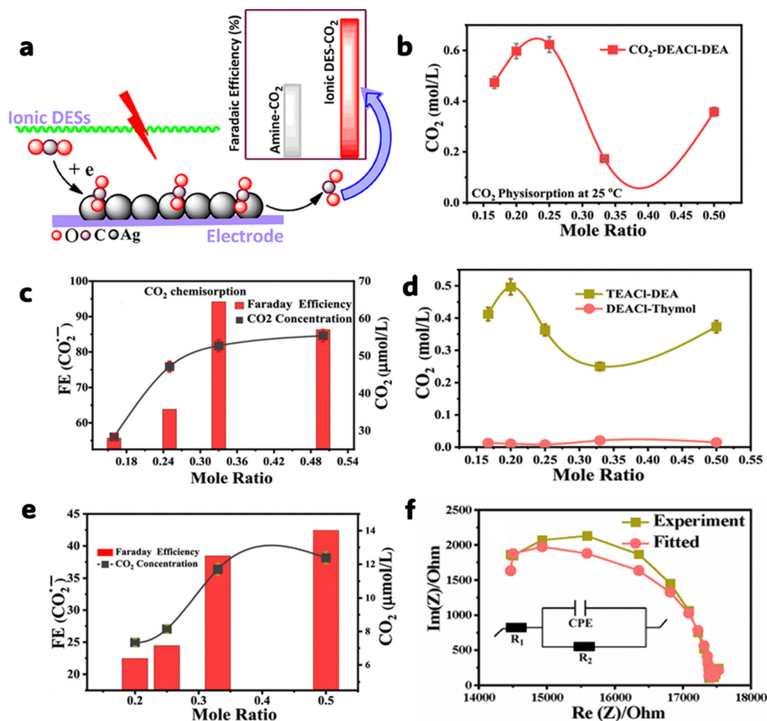
Fig. 66 (a) The graphical representation of CO 2 adsorption and electroreduction by DEACI-DEA. (b) Physiosorption of CO 2 by DEACI-DEA. (c) FE of CO 2 electroreduction to CO 2 . (d) Physiosorption of CO 2 by DEACI-thymol and TEACI-DEA. (e) FE of CO 2 electroreduction to CO 2 in TEACI-DEA where the secondary axis shows the amount of CO 2 chemisorbed. (f) Nyquist plot for CO 2 saturated DEACI-DEA. Reprinted (adapted) from ACS Omega 2022, 7(42), 37764–37773. Copyright © 2022, The Authors. Published by American Chemical Society under the terms of CC-BY-NC-ND 4.0 license.
