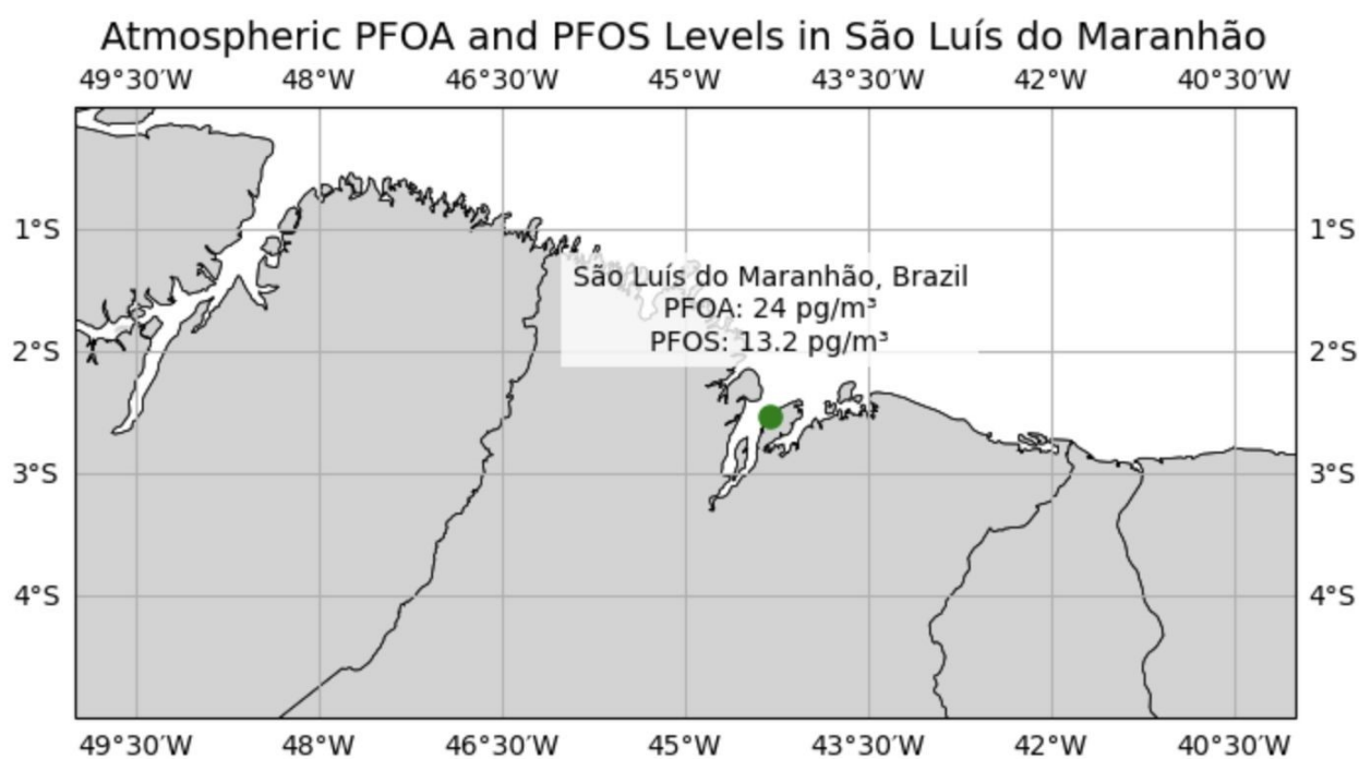
Figure 8 Atmospheric concentrations ( \text{pg}/\text{m}^3 ) of PFOA and PFOS in São Luís do Maranhão, as reported in prior work 106 . The map shows that the concentration of PFOA ( 24 \text{ pg}/\text{m}^3 ) is higher than that of PFOS ( 13.2 \text{ pg}/\text{m}^3 ).
