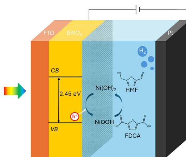
Fig. 2 Schematic illustration of the PEC system for HMF oxidation mediated by the \text{Ni}(\text{OH})_2/\text{NiOOH} redox couple.
