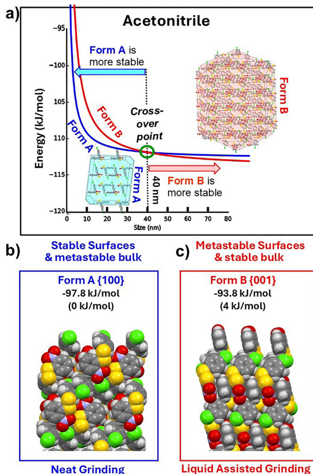
Fig. 31 Size-dependent polymorph stability. (a) Calculated stability cross-over at \sim 40 nm: Form A of 1-2 is favoured < 40 nm, Form B of 1-2 > 40 nm. (b) Form A of 1-2: stable surface, metastable bulk. (c) Form B of 1-2: metastable surface, stable bulk. 10 Adapted from ref. 10 with permission from The Royal Society of Chemistry.
