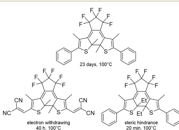
Fig. 2 Examples of thermal stability of DAE closed forms. 30
