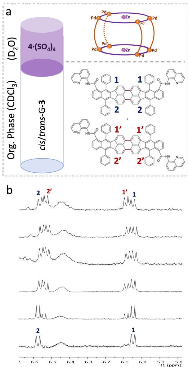
Fig. 2 (a) Schematic representation of the biphasic system designed to purify cis/trans -G-3 NGs. (b) Stacked partial 1 H NMR spectra of cis/trans -G-3 isomeric mixture, showing spectral changes upon selective host-guest complexation of trans -G-3 along the time (15 min intervals; time = 0, top spectrum; time = 75 minutes, bottom spectrum).
