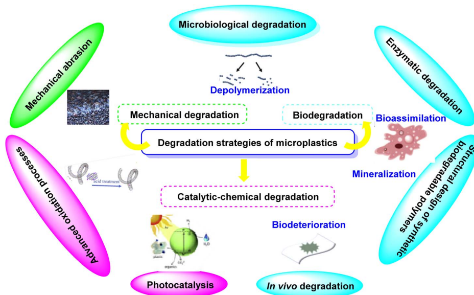
Fig. 8 Model diagram showing the pathways of MP degradation.
